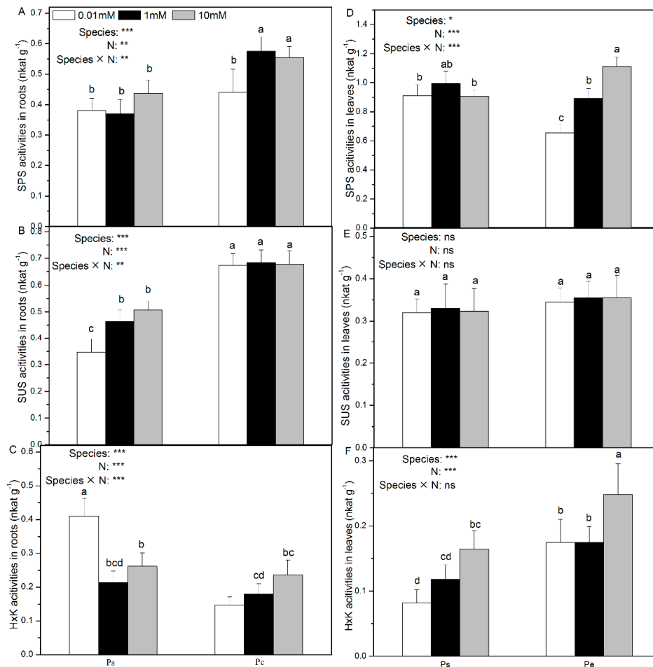
Figure 3. Sucrose phosphate synthase (A,D), sucrose synthase (B,E), and hexokinase (C,F) activities of P. simonii (Ps) and Populus euramericana (Pe) under 0.01, 1, and 10 mM \text{NH}_4\text{NO}_3 . Bars labelled with different letters indicate significant difference between the treatments. p -Values of the ANOVAs of species, N treatment, and their interaction are indicated. * p < 0.05 ; ** p < 0.01 ; *** p < 0.001 ; ns, not significant.
